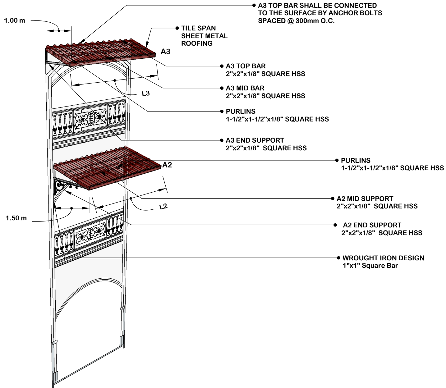
AWNING ELEVATION DETAILS
